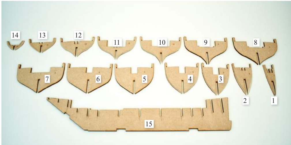
5 - Remove the bulkheads (91-14) from the 3mm MDF sheet, along with the keel (15). The front and rear bulkheads have an etched bevel line. You can rough bevel the edges of these bulkheads before slotting and gluing in place, meaning you do not have to bevel as much later.
