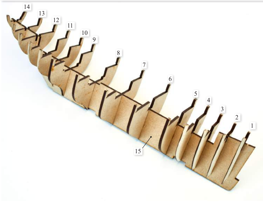
5 - Remove the bulkheads (91-14) from the 3mm MDF sheet, along with the keel (15). The front and rear bulkheads have an etched bevel line. You can rough bevel the edges of these bulkheads before slotting and gluing in place, meaning you do not have to bevel as much later.
