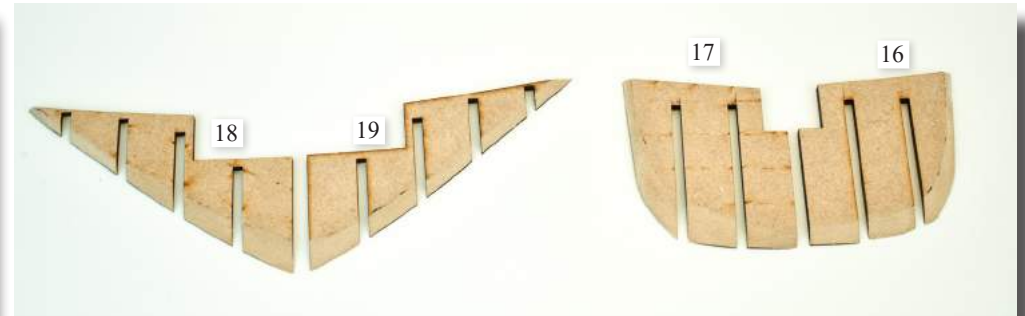
6 - Remove the fore filling patterns (16 & 17) and aft filling patterns (18 & 19) and bevel the edges to the marked bevel line as shown above. Slot and glue the fore patterns (16 & 17) in place as shown, followed by the stern patterns (18 & 19). Try not to glue areas of the patterns that are exposed, as the laser cut wooden stem and stern post are to be slotted in between the patterns.
