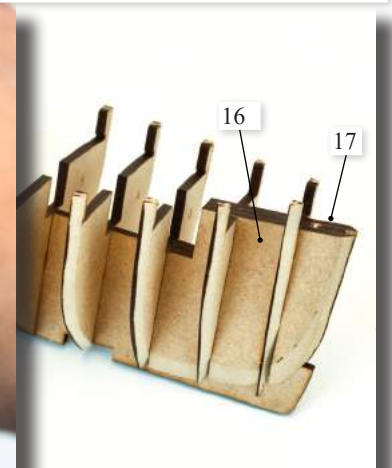
6 - Remove the fore filling patterns (16 & 17) and aft filling patterns (18 & 19) and bevel the edges to the marked bevel line as shown above. Slot and glue the fore patterns (16 & 17) in place as shown, followed by the stern patterns (18 & 19). Try not to glue areas of the patterns that are exposed, as the laser cut wooden stem and stern post are to be slotted in between the patterns.
