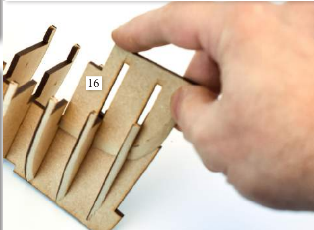
6 - Remove the fore filling patterns (16 & 17) and aft filling patterns (18 & 19) and bevel the edges to the marked bevel line as shown above. Slot and glue the fore patterns (16 & 17) in place as shown, followed by the stern patterns (18 & 19). Try not to glue areas of the patterns that are exposed, as the laser cut wooden stem and stern post are to be slotted in between the patterns.
