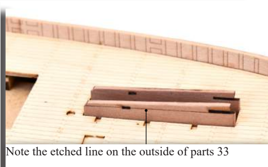
21 - Below - Remove the parts that make up the fore mast housing. Take note, parts 33 are handed, and the laser engraved line should be on the outside face of each pattern. Slot and glue parts 33 into position in the fore deck and into the slots located in the lower platform.
