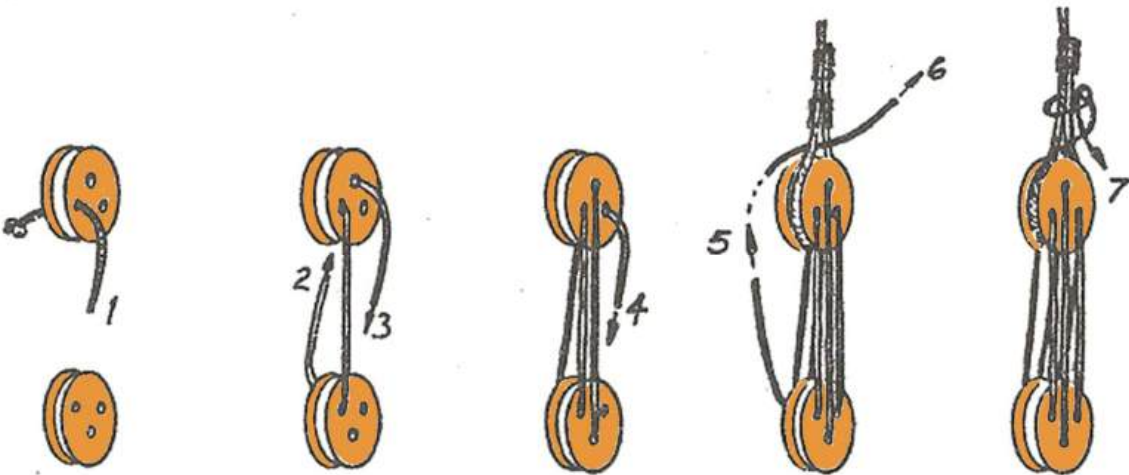
Reeving Deadeyes
