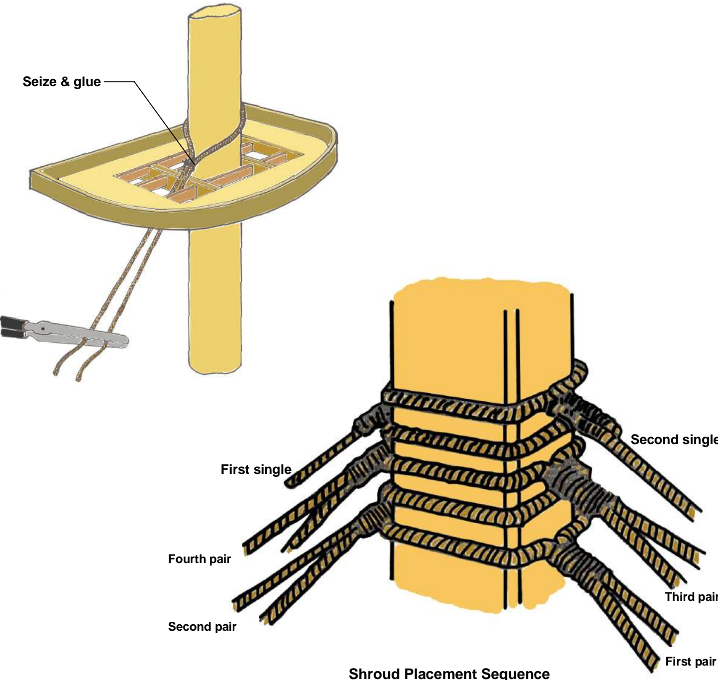
Shroud Placement Sequence
