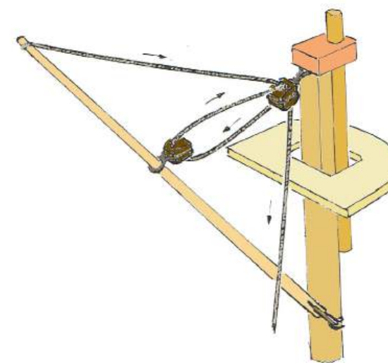
Reeving Blocks
